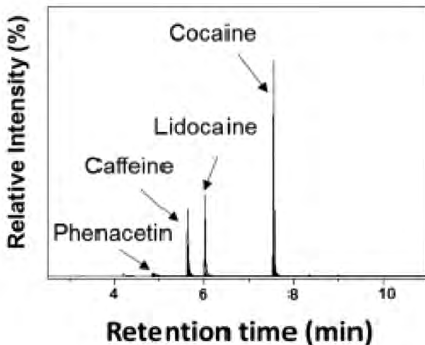
Obr. 3: Chem. profil kokainu ve formě chromatogramu (Zdroj: http://ars.els-cdn.com/content/image/1-s2.0-S1355030615001409-gr4.jpg )
