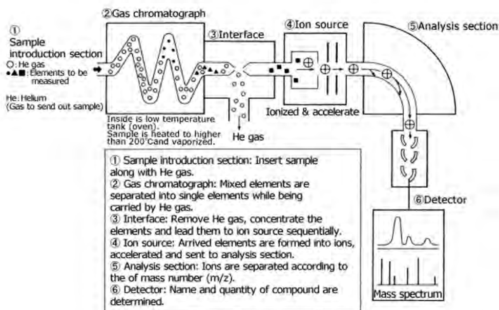
Obr. 2: Princip GC-MS (Zdroj: https://www.jeol.co.jp/en/science/product_file/file/en_sc17-3.gif )
